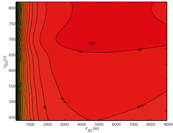
3D efficiency diagram for blueplanet 9.0 TL3
